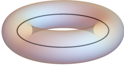
Figure 5. An illustration of a toroidal surface that wraps a circular defect.
