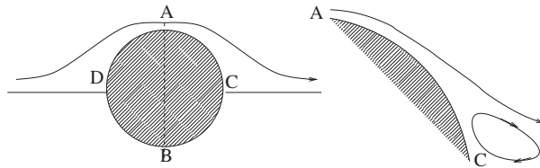
Figure 1: Symmetric streamlines for an ideal flow (left) and appearance of separation and a recirculating vortex in a viscous fluid (right).
